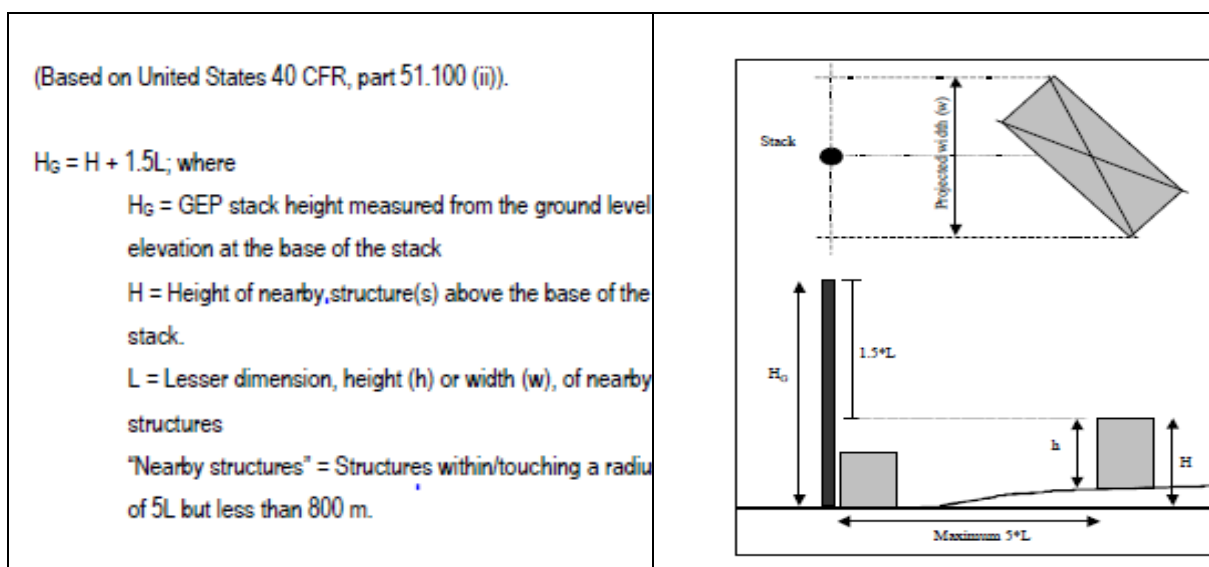
Figure 1-2: Stack Height design for Incinerator Chimney
